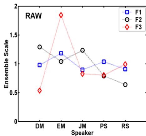
Figure 6: Per-formant profile of RAW scales for the 5 speakers. “RAW” signifies that the scales shown are based simply on the original (token-averaged) PSEs.
